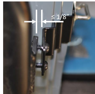
Figure 16: Installed Weather Stripping After Modification
