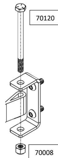
Figure 22: Door Stop Anchor Hardware
